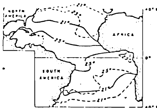
Fig. 3 Average winter (—) and summer (---) surface isotherms ( ^{\circ}\text{C} ) in the Atlantic Ocean (after Sverdrup et al., 1942). Areas with prolonged exposures to temperatures less than 22^{\circ}\text{C} , or with short exposures less than 18^{\circ} , at best will have a depauperate coral population. Periodic influxes of cold waters from the Guinea Current have helped to severely limit reef development off tropical Africa.
