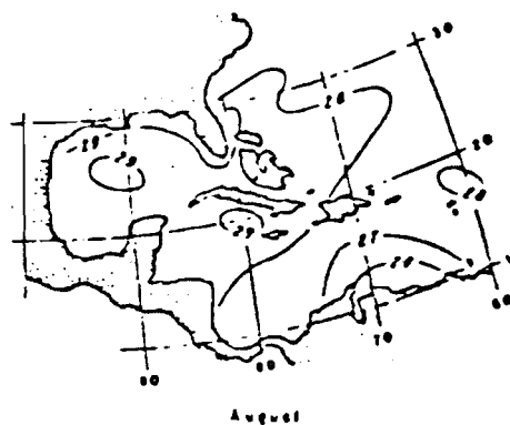
Fig. 4 Average winter (February) and summer (August) surface temperatures ( ^{\circ}\text{C} ) in the Caribbean (after Sverdrup et al., 1942).
